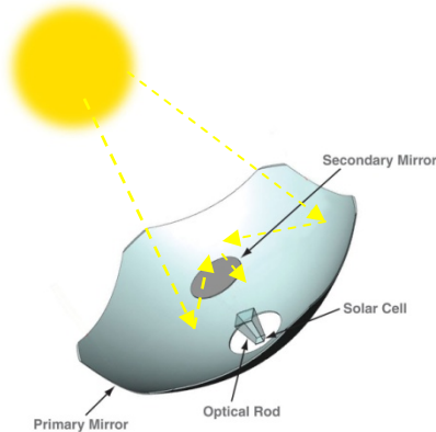
In the diagram above, a reflective, mirror-based optical system is used for concentration. The sun's light is collected by the primary mirror, which focuses the light onto the secondary mirror, which concentrates light onto the photovoltaic cell located at the base of the optical rod.
